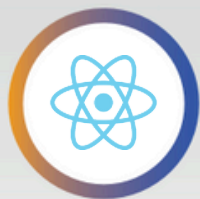
React Native
